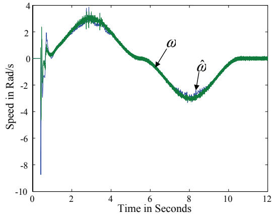
Figure 1: \omega and \hat{\omega} in rad/sec vs. time in seconds with full load on the motor.
