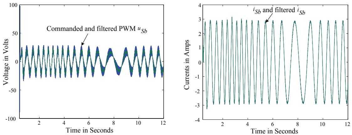
Figure 2: Left: u_{sb} commanded and filtered. Right: i_{sb} measured and filtered.
