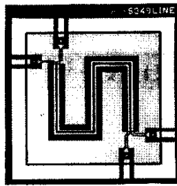
Fig. 5. Microphotograph of a fabricated 3-dB coupler.
