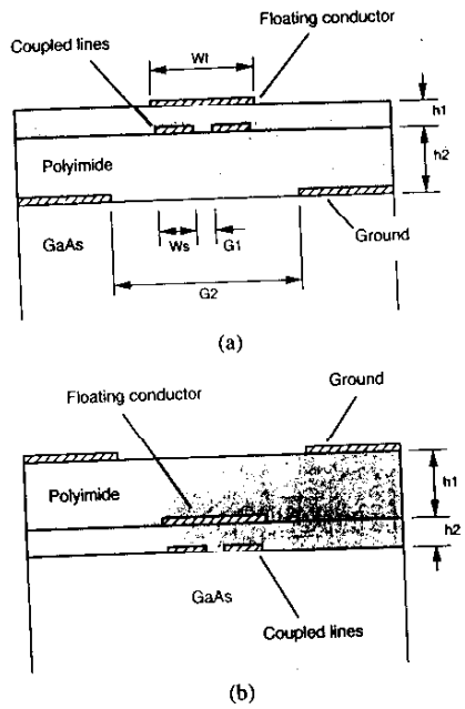
Fig. 1. Cross-sectional views of multilayer MMIC directional couplers. (a) Normal type and (b) inverted type.
