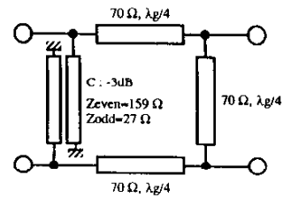
Fig. 7. Circuit diagram of a reverse-phase hybrid ring.
